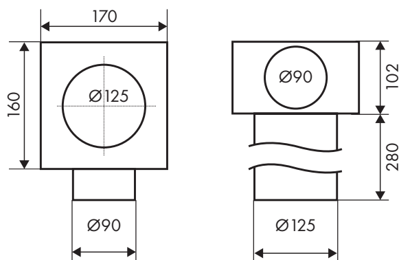
FLEXO BOX PRO T1 — 1×Ø90/Ø125
