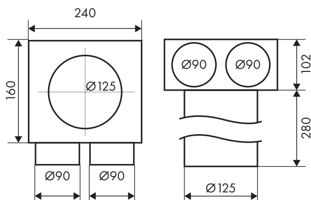
FLEXO BOX PRO T2 — 2×Ø90/Ø125
