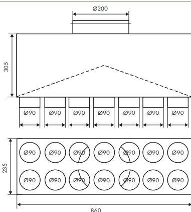
FLEXO BOX PRO P14x90/200
